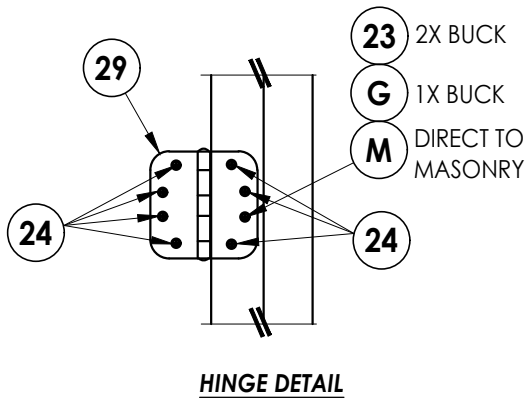
HINGE DETAIL
