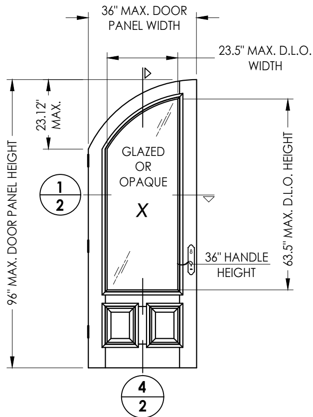
40 WOOD DOOR PANEL Glazed or Opaque
