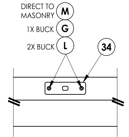
DETAIL 1 Astragal Shootbolt Strike Plate @ Head
